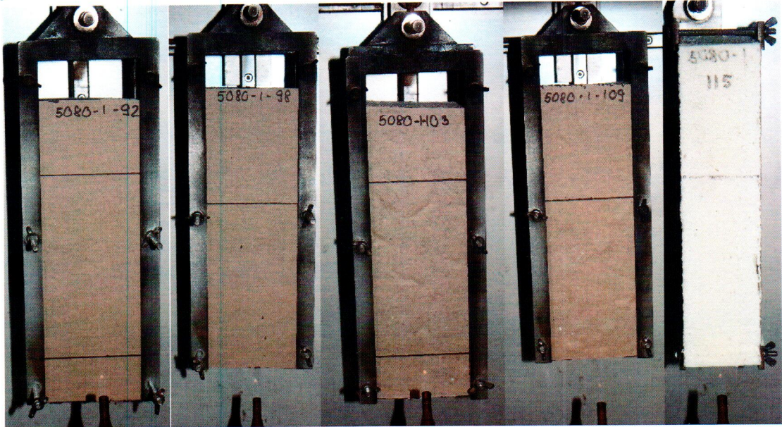
Fig. 1. Ignitability test (flame application to surface, bottom edge and side bottom edge).
