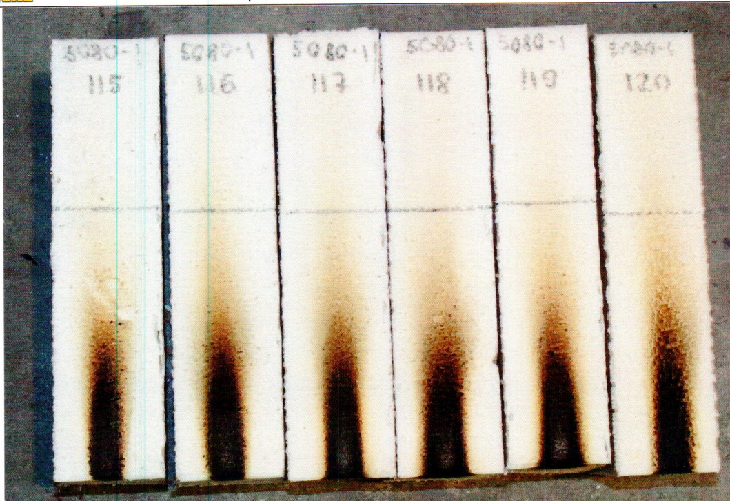
Fig.4. Specimens with 60 mm thickness after tests.
